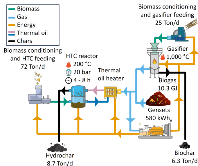
Figure 3 - General process flow diagram, PCH-CDMX Phase I. Source: Author's own elaboration.
